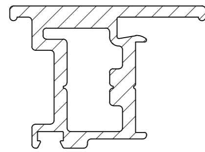
Profile A39595 1m=1,53 kg Material: aluminium
