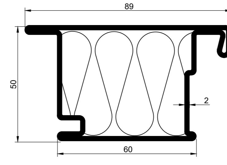
Profile P214868 1m=4,80 kg Material: steel | Material: stal
