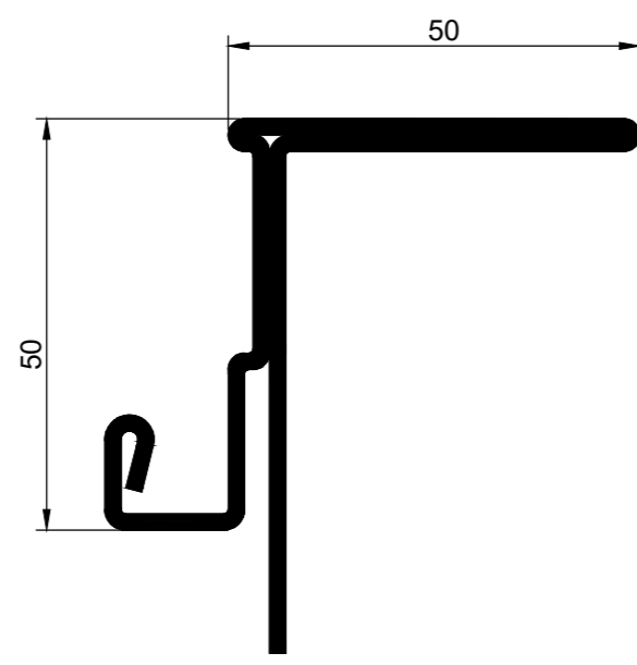
Profile P215700 1m=3,76 kg Material: steel | Material: stal
