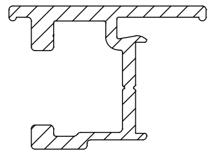
Profile A4195 1m=1,35 kg Material: aluminium
