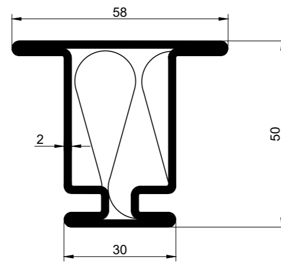
Profile P18364 1m=3,74 kg Material: steel | Material: stal
