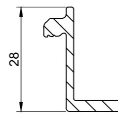
Profile A9840 1m=0,27 kg Material: aluminium
