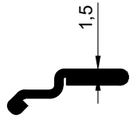
Profile P18144 1m=0,45 kg Material: steel | Material: stal
