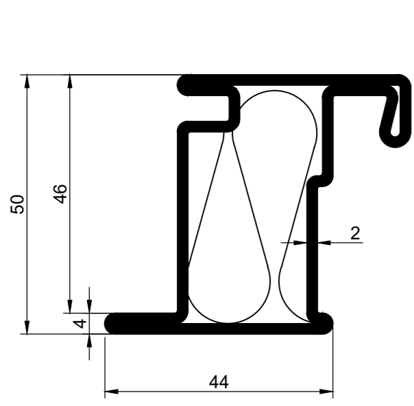
Profile P214867 1m=3,85 kg Material: steel | Material: stal
