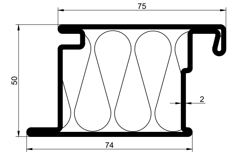
Profile P214514 1m=4,80 kg Material: steel | Material: stal
