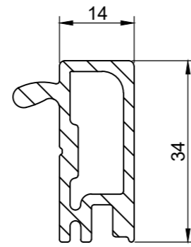
Profile A39553 1m=0,68 kg Material: aluminium
