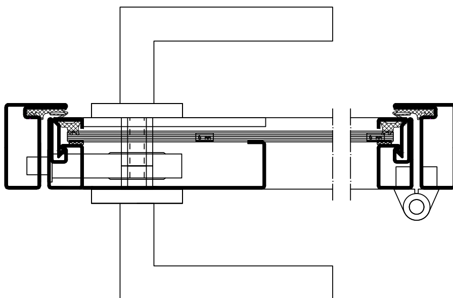
horizontal section of the door type A20
