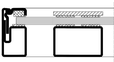
Aluminium + steel 40 [mm]
