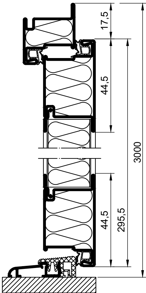
vertical section of the door type 099
