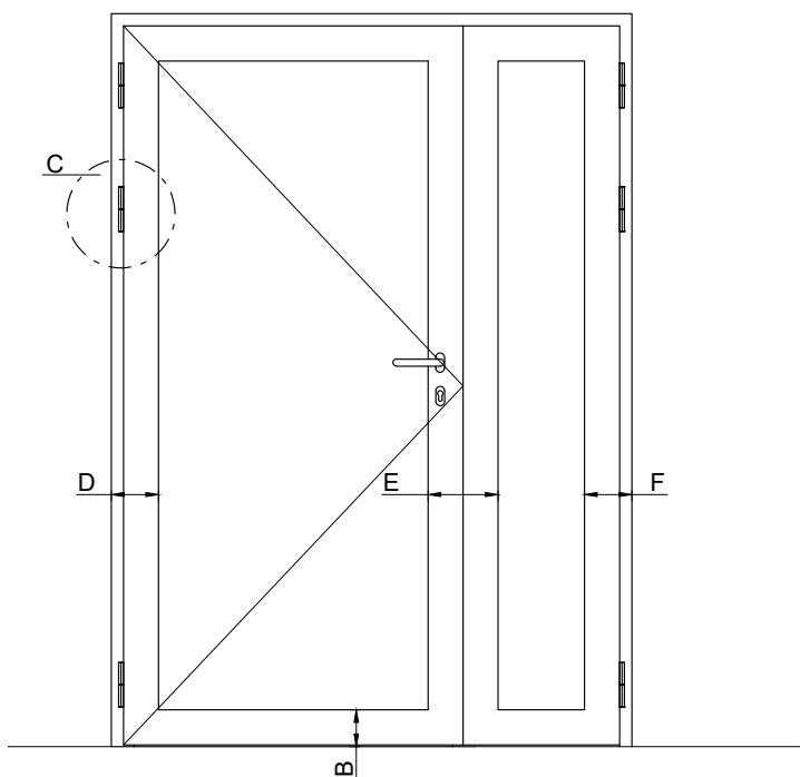
view of the door type TB40
