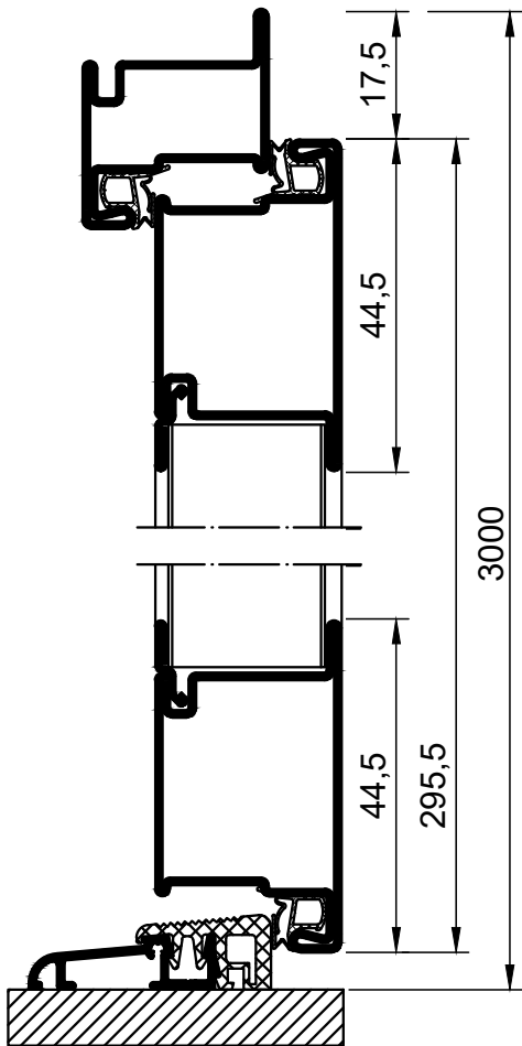
vertical section of the door type 43
