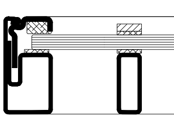
Aluminium + steel 10 [mm]
