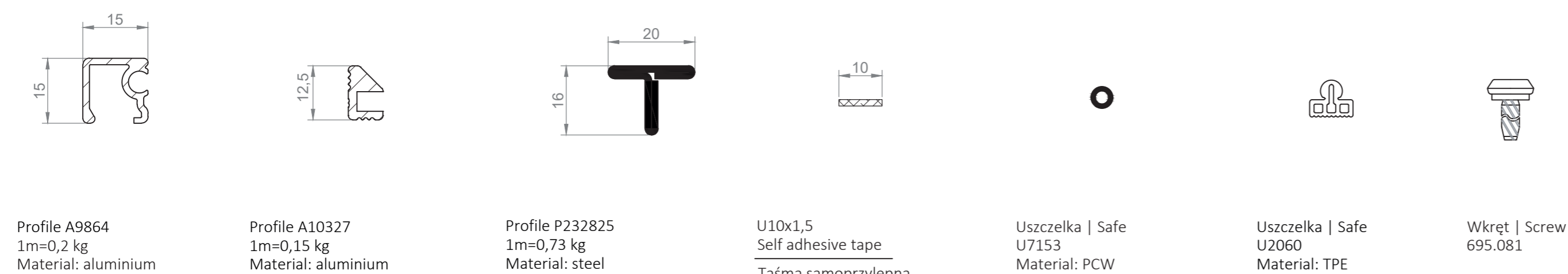
Cross-section example 1
