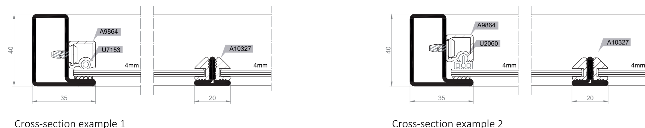
Cross-section example 1
